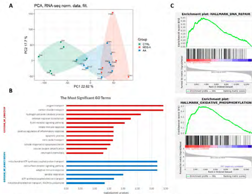
Figure 1: A) Principal component analysis of AA, MDS-h, and control RNA-Seq data. B) Gene Ontology (GO) functional analysis of significantly upregulated (red) and downregulated (blue) genes in T cells from patients with AA and MDS-h. C) GSEA plots for HALLMARK gene sets: DNA Repair and Oxidative Phosphorylation (controls vs. patients).
