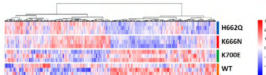
Figure 2. Heatmap of expression changes of all mitochondria-related genes in four isogenic NALM6 cell lines. Red – upregulation, blue – downregulation.
